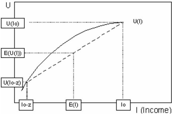
Figure 1 The demand for insurance (p=0.5)
