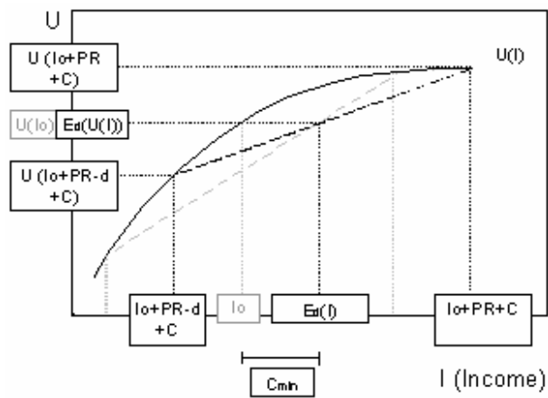
Figure 4 The minimum compensation ( p=0.5 )
