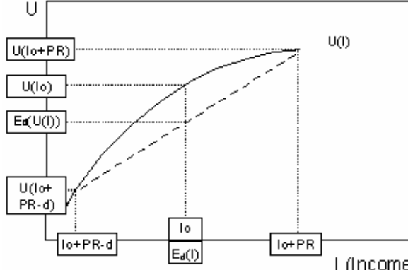
Figure 3 The demand for deductibles (p=0.5)
