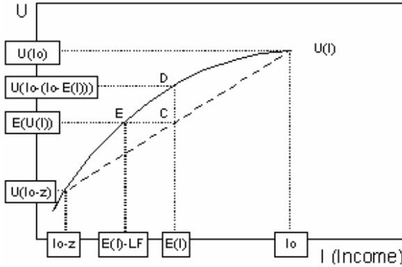
Figure 2 The maximum loading fee (p=0.5)
